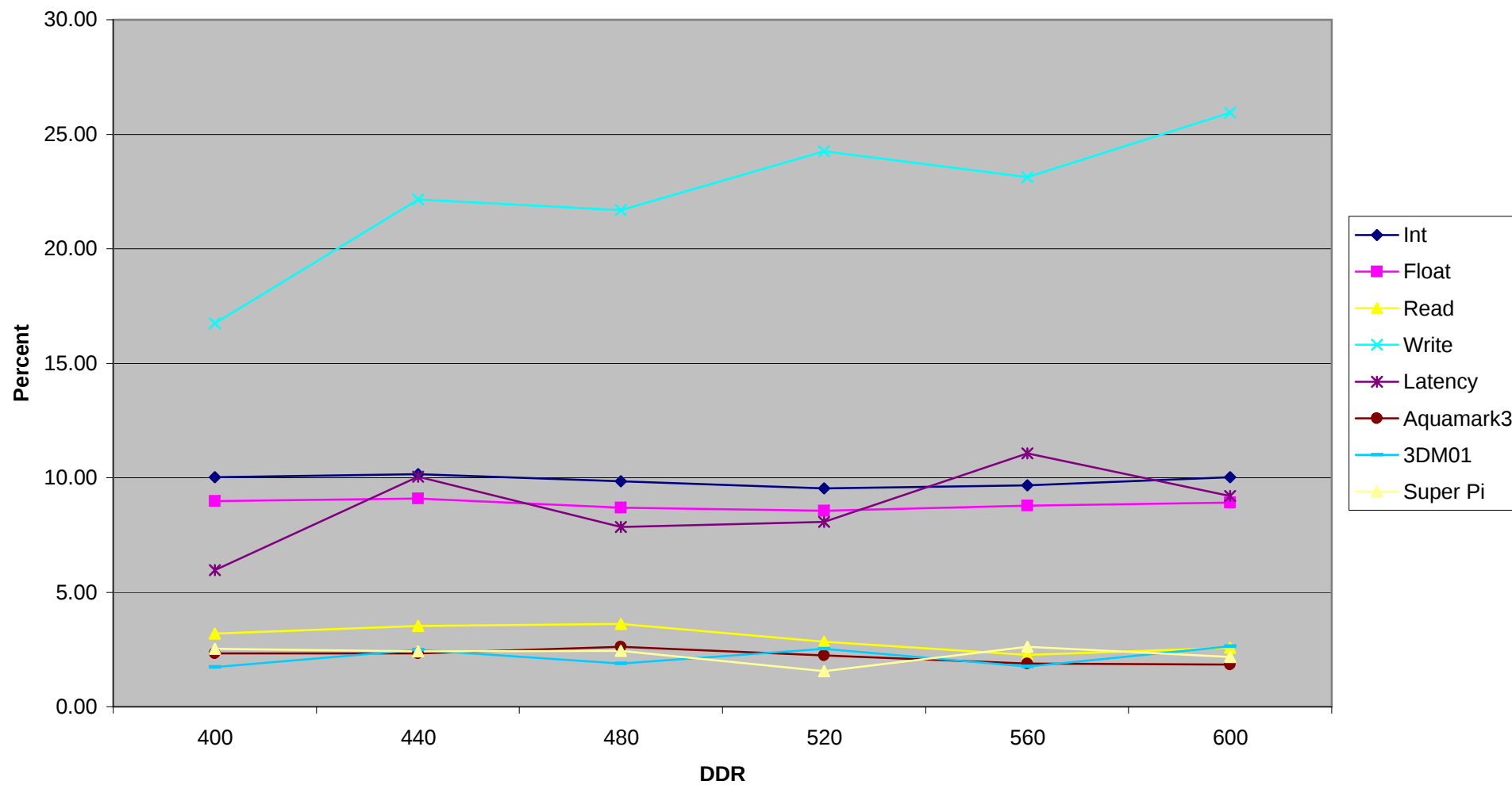
1T vs 2T Comparison (A64 3000+ Venice x9 1:1 @ 2.5-4-4-7)
